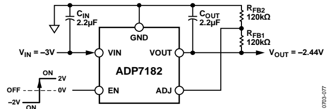
Figure 79. Setting Adjustable Output Voltage
