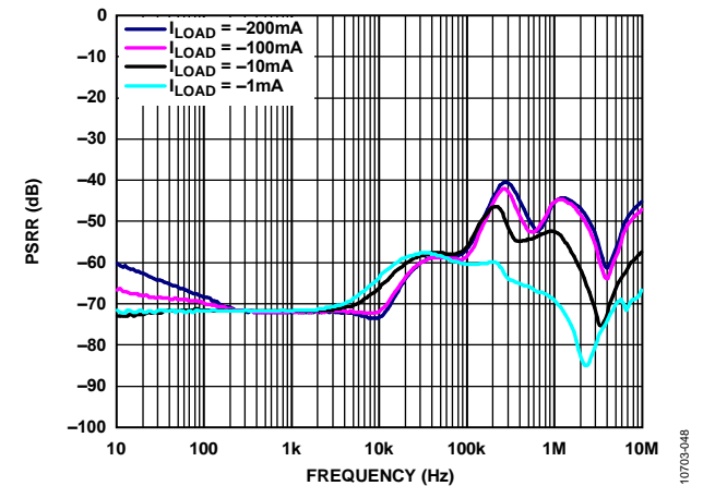
Figure 50. Power Supply Rejection Ratio (PSRR) vs. Frequency, V_{OUT} = -1.22 V vs. Different Load Currents ( I_{LOAD} ), V_{IN} = -5.7 V
