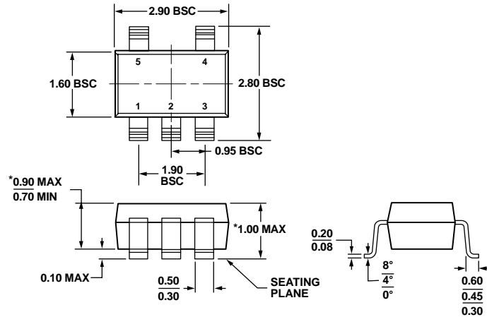
Figure 106. 5-Lead Thin Small Outline Transistor Package [TSOT] (UJ-5)
