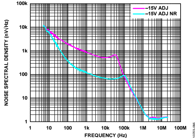
Figure 88. -15\ \text{V} Adjustable ADP7182 with and without the Noise Reduction Network ( C_{NR} and R_{NR} )
